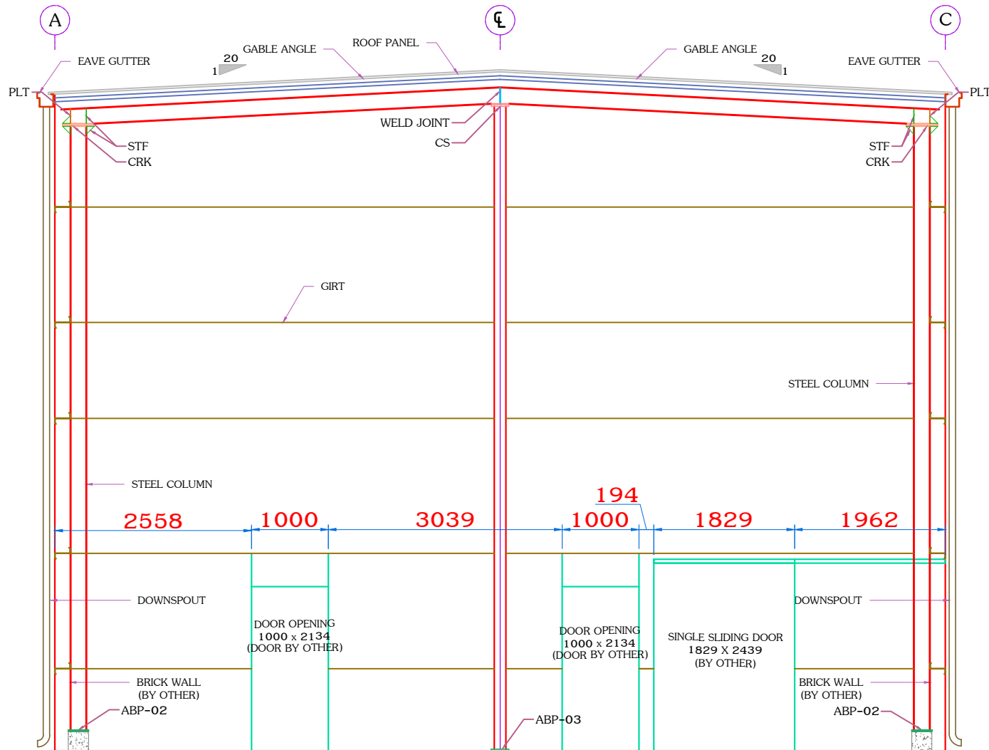
END WALL FRAMING @ GRID-1
